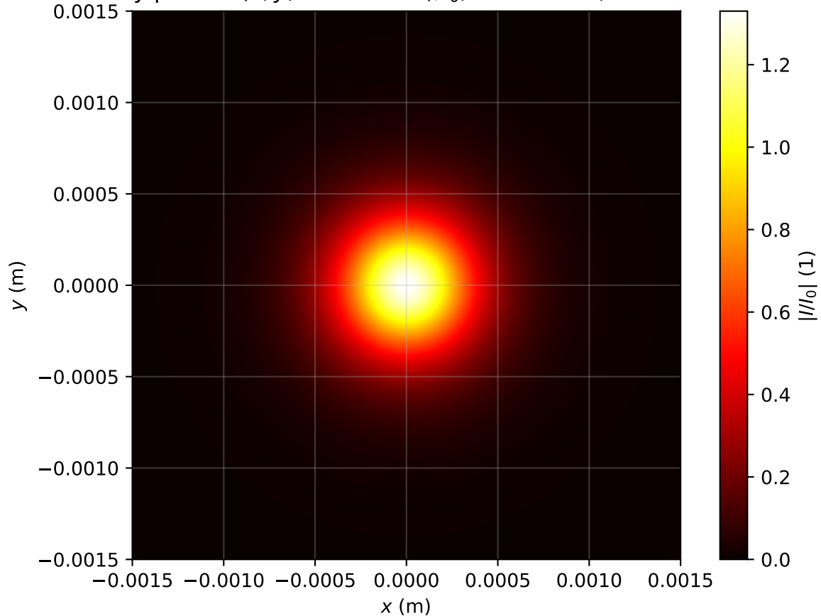
Intensity profile I(x, y, z = 1.911m)/I_0 , P_{in}=0.8P_{cr} , artificial time
